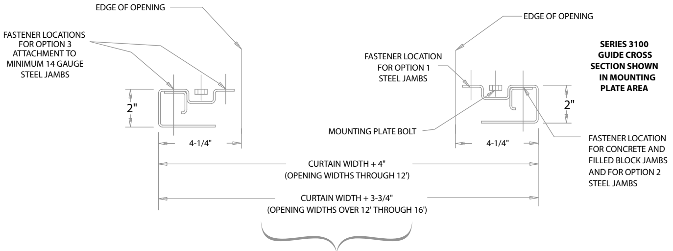
FIGURE 3 GUIDE INSTALLATION
