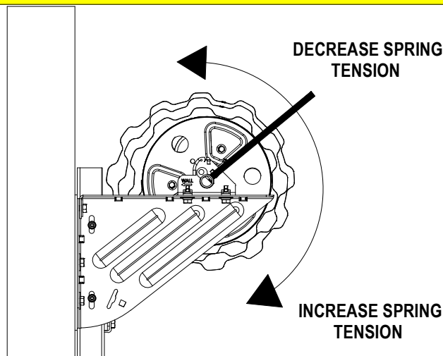
FIGURE 23: ADJUSTING SPRING TENSION
